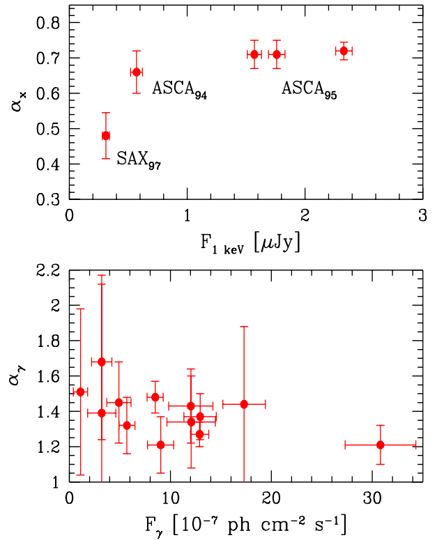
Fig. 5. Spectral indices vs flux in the [2–10] keV and [0.05–1] GeV bands. All X-ray data have been reanalysed assuming a fixed N_{\text{H}} = 5.3 \times 10^{21} \text{ cm}^{-2} . \gamma -ray data from Mukherjee et al. 1996, 1997a, 1997b, 1999.
